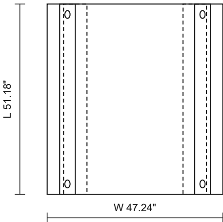
BOTTOM (UNDERSIDE)
