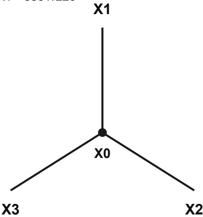
SECONDARY - 380Y/220
