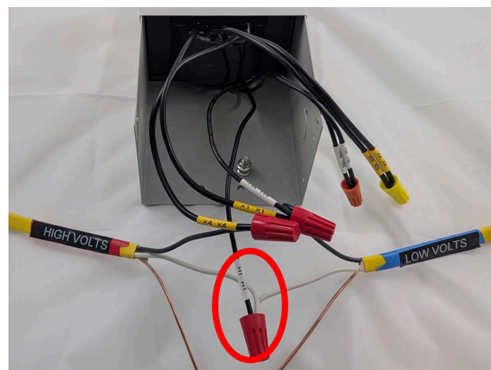
Step 5 Connect High & Low Voltage L2 to H1
