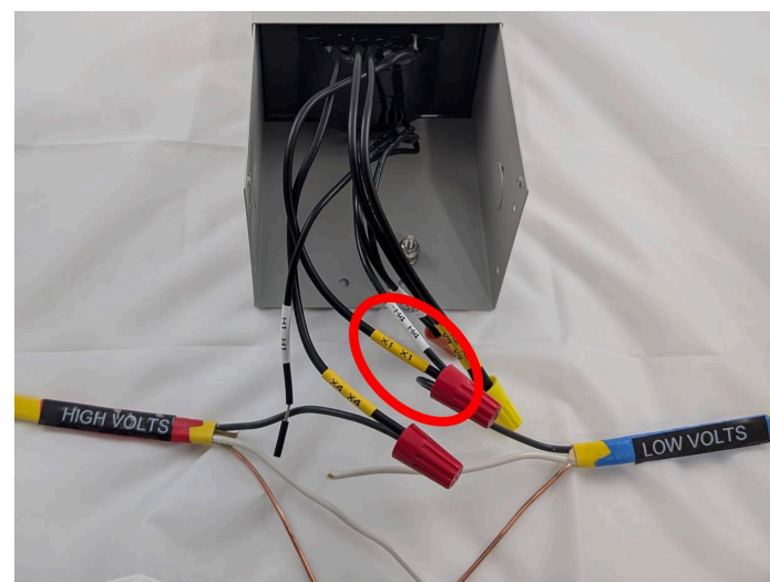
Step 4 Connect Low Voltage L1 to H4 and X1
