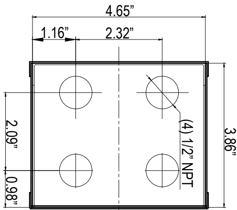
(4) 1/2" NPT Knockouts Bottom (Underside) Plate
