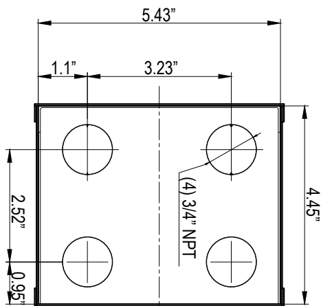
(4) 3/4" NPT Knockouts Bottom (Underside) Plate
