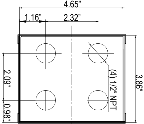
(4) 1/2" NPT Knockouts Bottom (Underside) Plate
